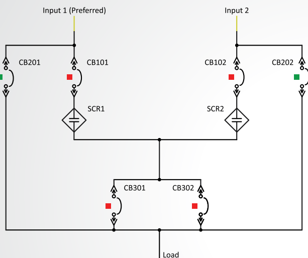
eSTS Static Transfer Switch One Line Diagram
